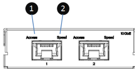
Figure 2-21 2-port 10 GBASE-T iSCSI Host Card (RJ45) LEDs
