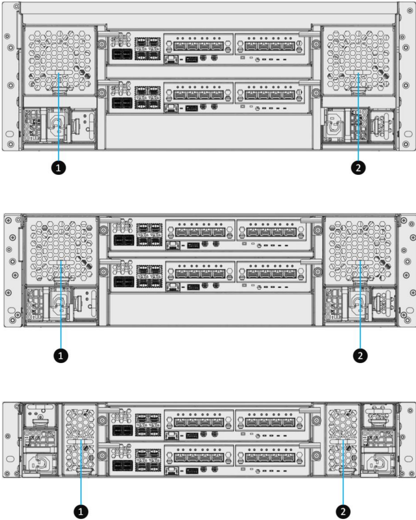
Figure 2-9 Location of the Fan Modules
